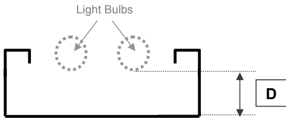
End View of Lens
