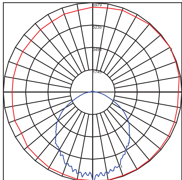
Maximum Candela = 6979.49 Located At Horizontal Angle = 30, Vertical Angle = 1 # 1 - Vertical Plane Through Horizontal Angles (30 - 210) (Through Max. Cd.) # 2 - Horizontal Cone Through Vertical Angle (1) (Through Max. Cd.)
